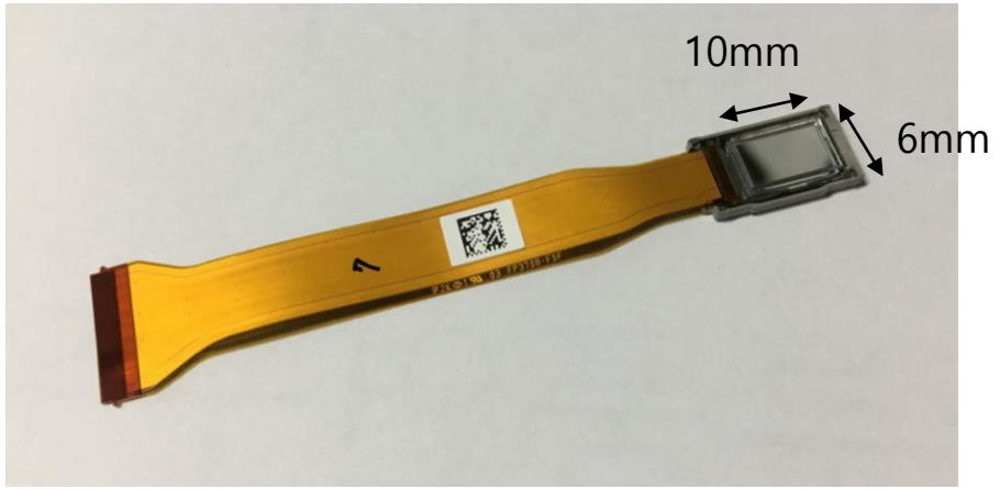
SXRD241AZ-6(0.94cm Silicon Reflective Liquid Crystal Display) 1920(H)x1080(V) / 4.3um pixel pitch3DOT
